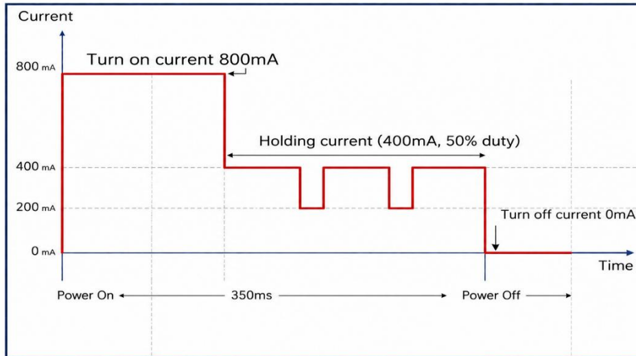
Topology Example (50% duty)
