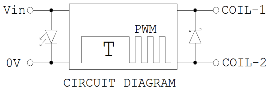
Surge Protection, LED x 1(power on)
